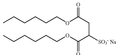
di-C 6 SS, sodium bis(hexyl)sulfosuccinate
