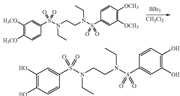
N,N'-Diethyl-N,N'-bis-(3,4-dihydroxybenzosulfonyl)-1,2-ethylenediamine
