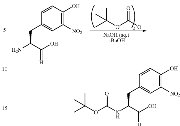
tert-Butyloxycarbonyl-3-nitro-L-tyrosine
