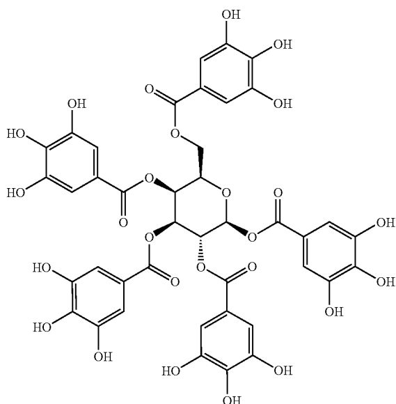
\beta -D-Galactopyranose Pentakis[3,4,5-trihydroxybenzoate]
