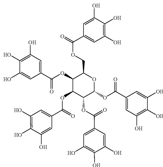
\alpha -D-Galactopyranose Pentakis[3,4,5-trihydroxybenzoate]
