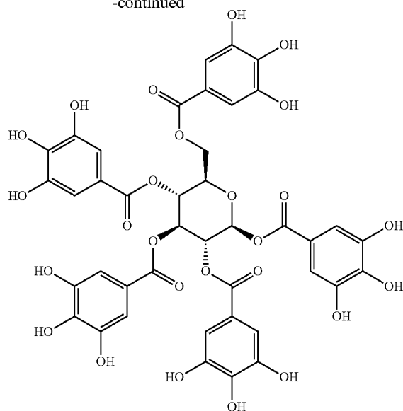
\beta -D-Glucopyranose Pentakis[3,4,5-trihydroxybenzoate]
