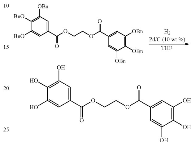
1,2-Bis-galloyloxyethane
