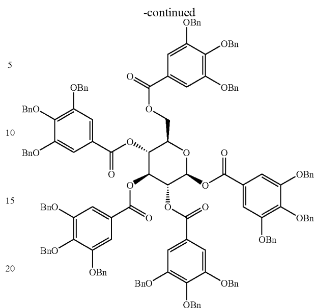
\beta -D-Glucopyranose Pentakis[3,4,5-tris(phenylmethoxy)-benzoate]
